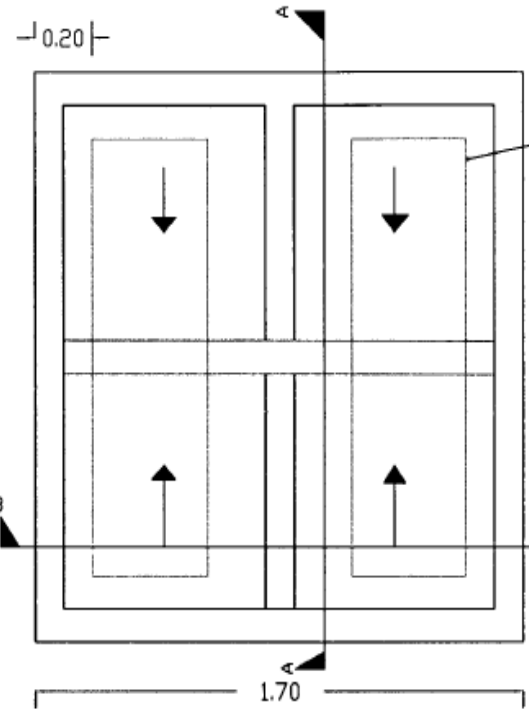
4-compartment cloth washbasin plan
