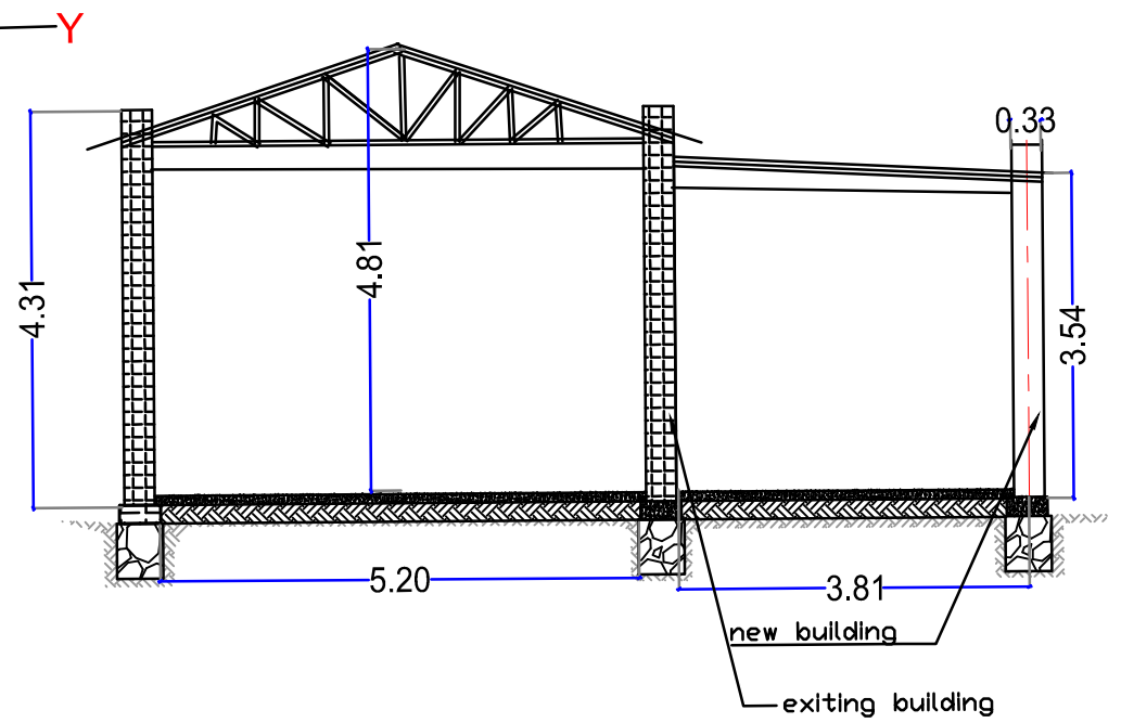
Y-Y section Details
