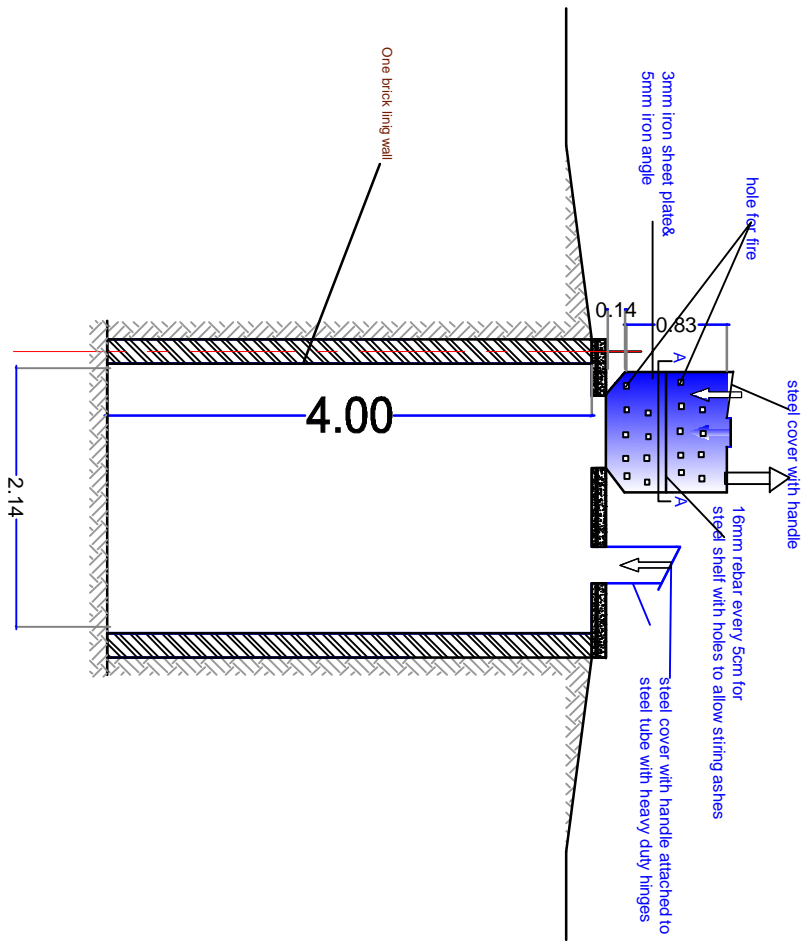
X-X SECTION VIEW
